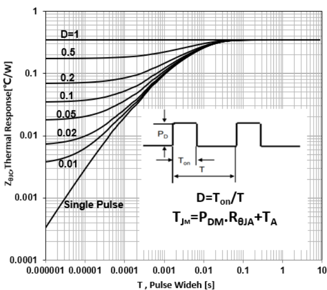
Figure 11. IGBT Transient Thermal Impedance vs Pulse Width
