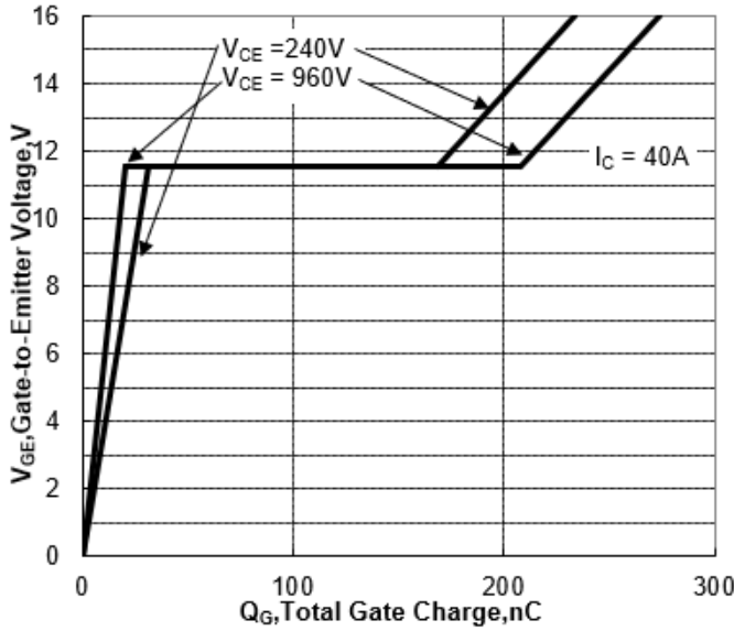
Figure 9. Typical Gate Charge
