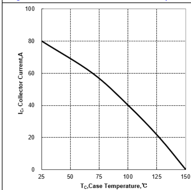
Figure 3. Collector Current vs Case Temperature
