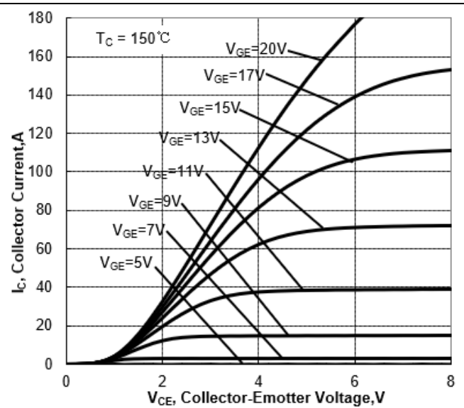
Figure 6. Typical Output Characteristics( T=150^{\circ}\text{C} )
