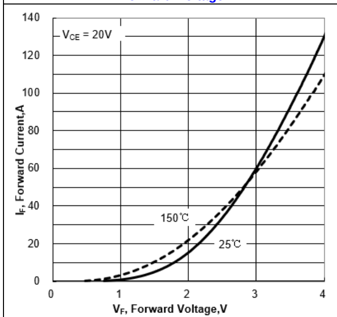
Figure 13. Typical Diode Forward Current vs Forward Voltage
